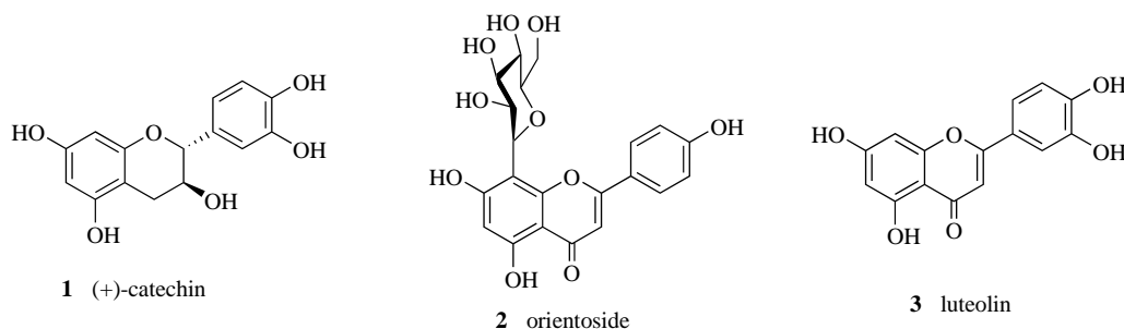
Fig. 1 Structures of compounds 1-3
