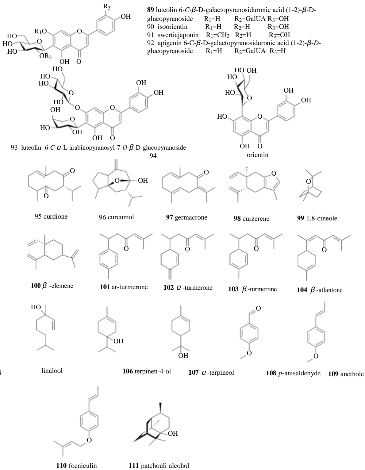
Fig. 12 Structures of compounds 89-111
