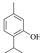
125 thymol
