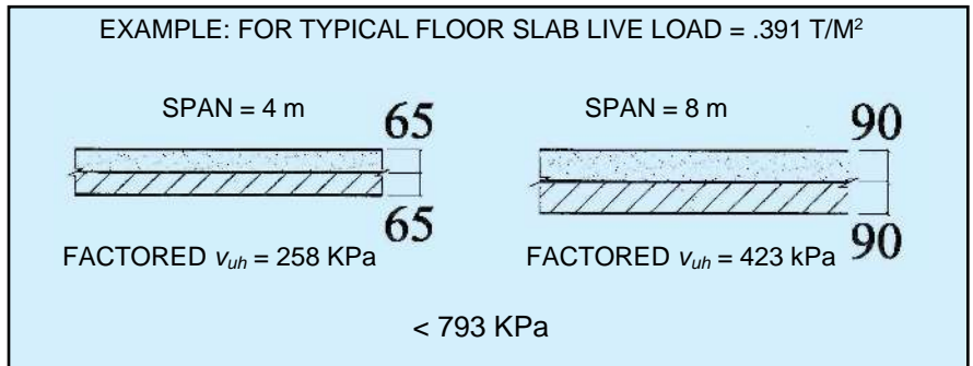
Fig. 8. Calculated horizontal shear stresses for a composite slab under ordinary loading conditions.
