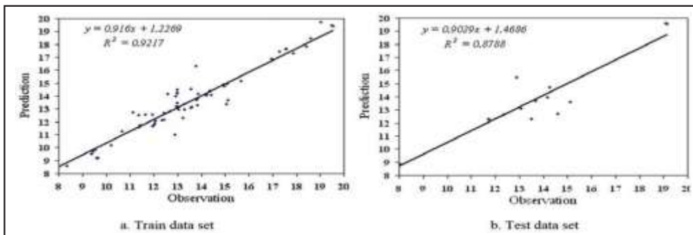
Figure 7. Scatter plot of predicted vs. observed values of Compressive Strength for BPNN (5-7-2)
