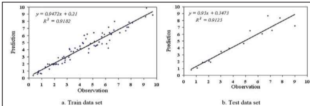
Figure 6. Scatter plot of predicted vs. observed values of Permeability for BPNN (5-7-2)
