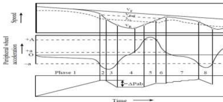
Figure.8. ABS algorithm
