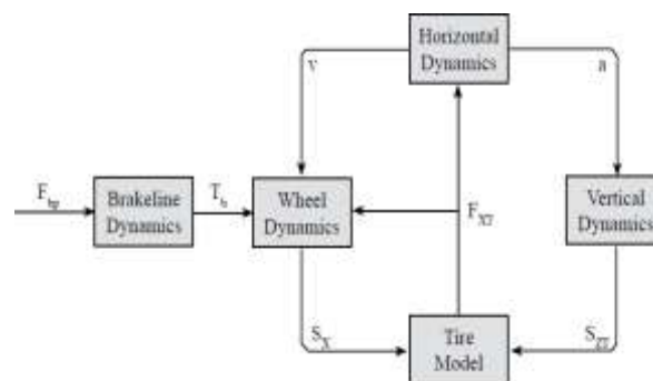
Figure.7. Vehicle dynamics Overview
