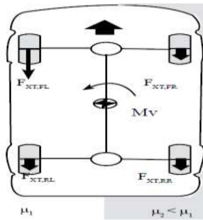
Figure.2 Buildup of yaw moment induced by large differences in friction coefficients.
