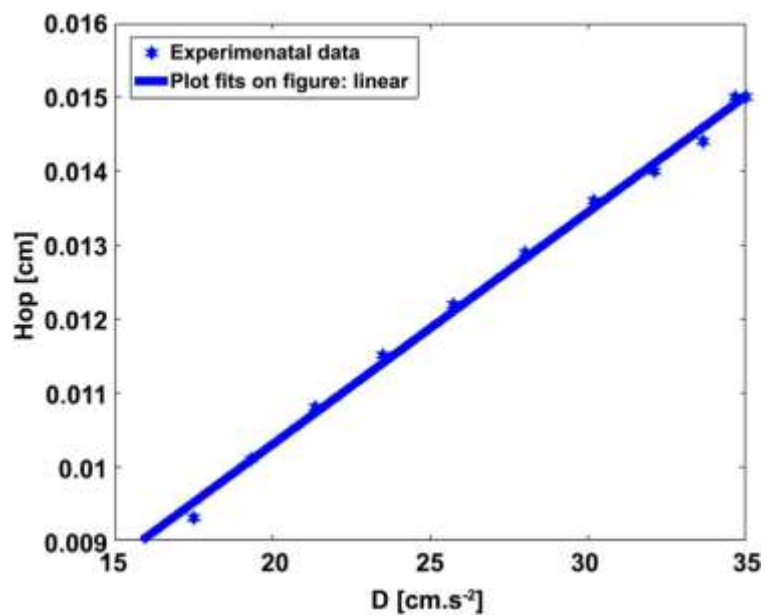
Figure 6. Optimum thickness versus diffusion coefficient.
