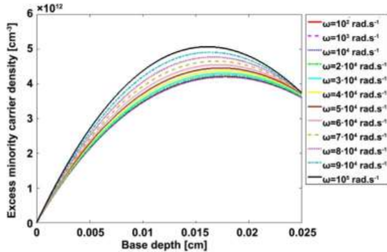
Figure 2. Excess minority carrier density versus base depth for different frequencies ( D_0 = 35 \text{ cm} ; \alpha = 6.2 \text{ cm}^{-1} ).
