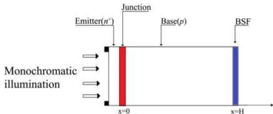
Figure 1. Structure of n^+ -p/ p^+ silicon solar cell.
