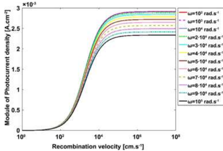
Figure 3. Module of photocurrent density versus recombination velocity for different frequency ( D = 35 \text{ cm} ; \alpha = 6.2 \text{ cm}^{-1} ).
