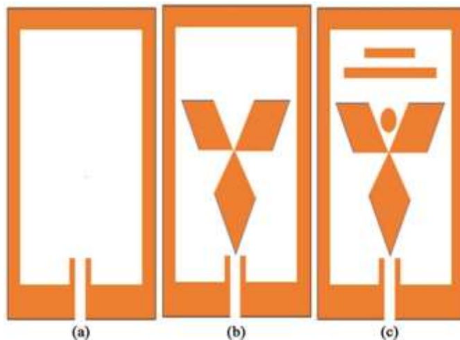
Figure 1. Initial (a) second (b) and final (c) structure of the antenna.
