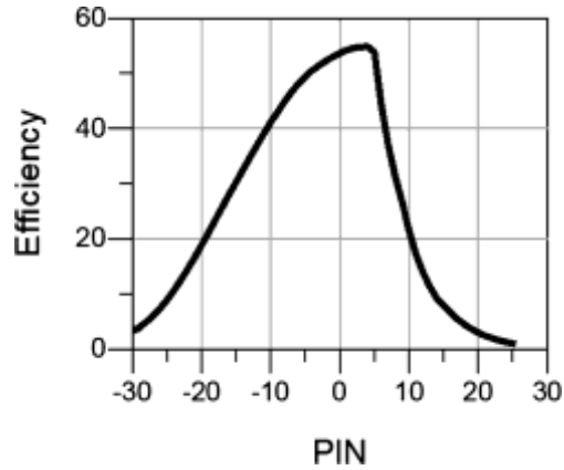
Figure 8. Single band rectifier: RF-to-dc conversion efficiency versus input power (dBm).
