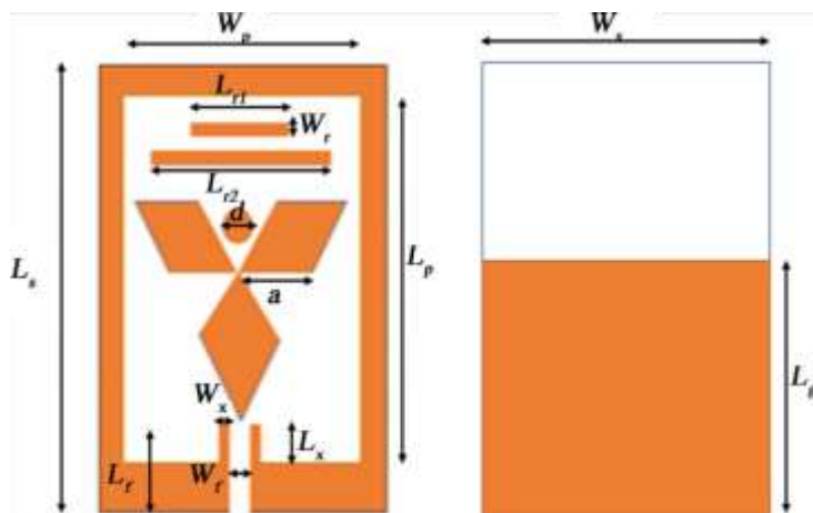
Figure 2. Proposed antenna.
