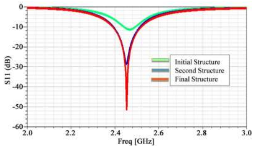
Figure 3. Reflection coefficient variation from initial to final structure.
