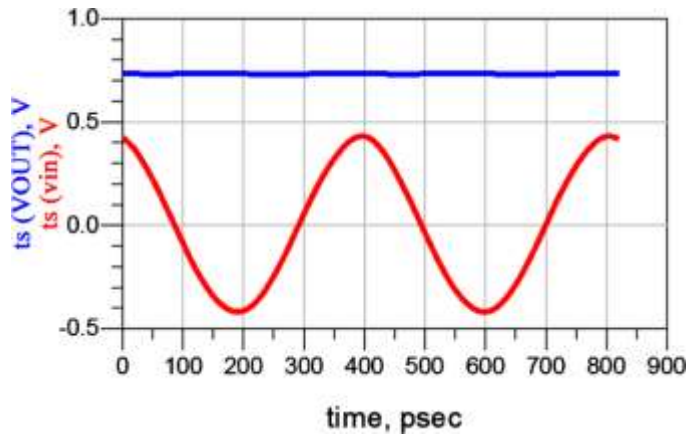
Figure 9. Simulated input and output voltage.
