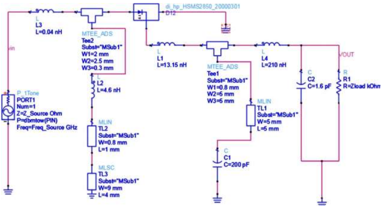
Figure 6. Simulation of the adaptation and rectification circuit.
