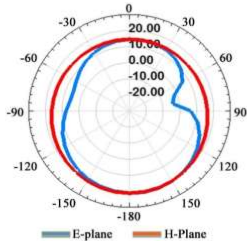
Figure 5. Radiation patterns of the antenna at 2.45 GHz.
